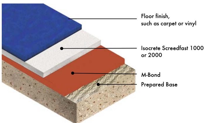
TYPICAL SECTION SHOWING SCREDFAST BONDED WITH EPOXY BONDING AGENT (M-BOND)
